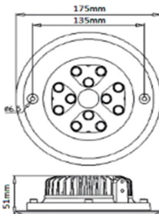
Cutting: Ø155
